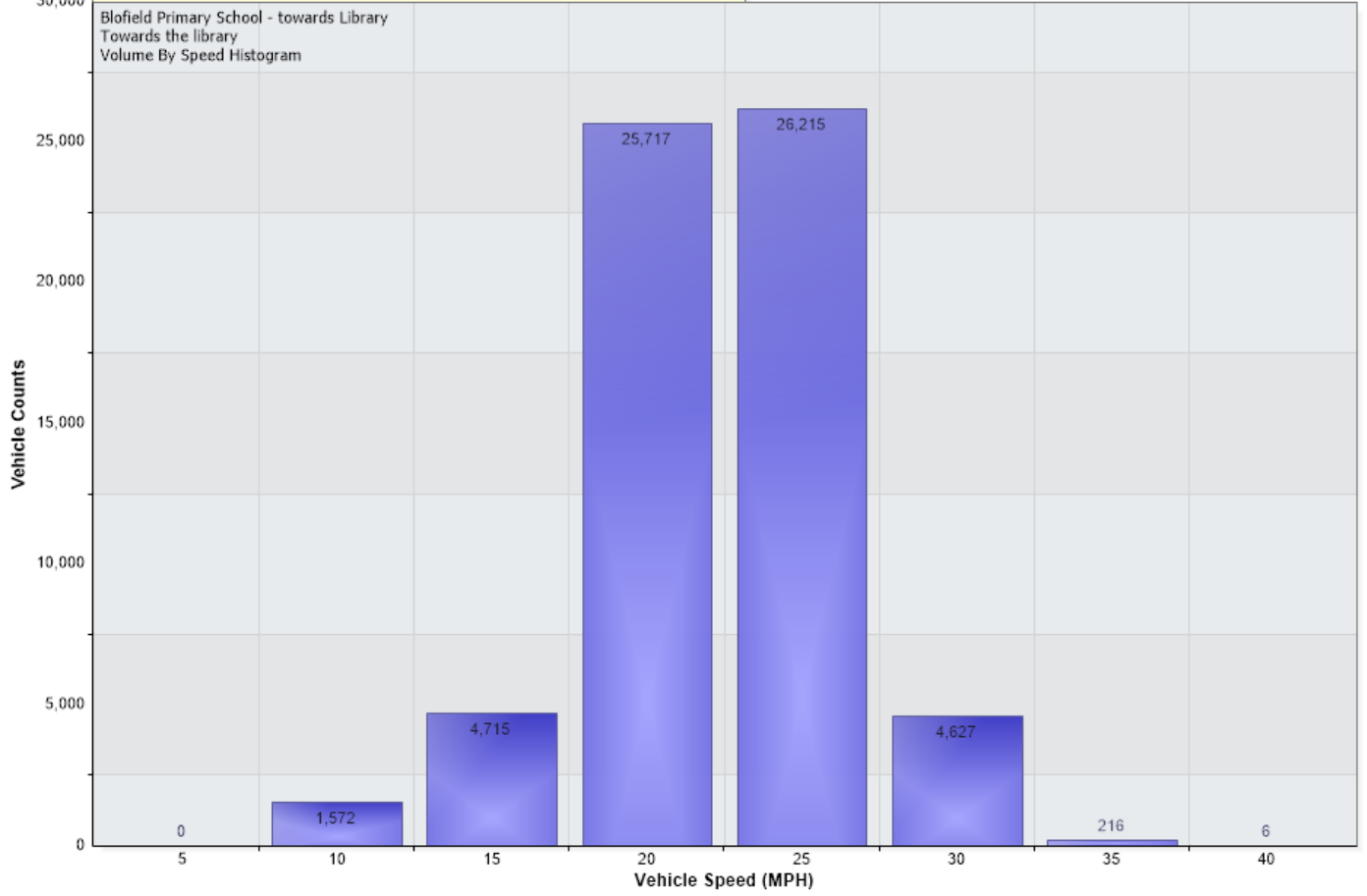
Vehicle Counts Vs. Speed [Blofield Primary School - towards Library: Incoming]
